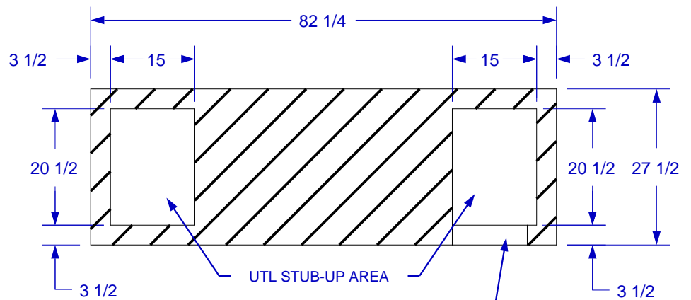
STUB-UP DIAGRAM (SEE NOTE #2)
