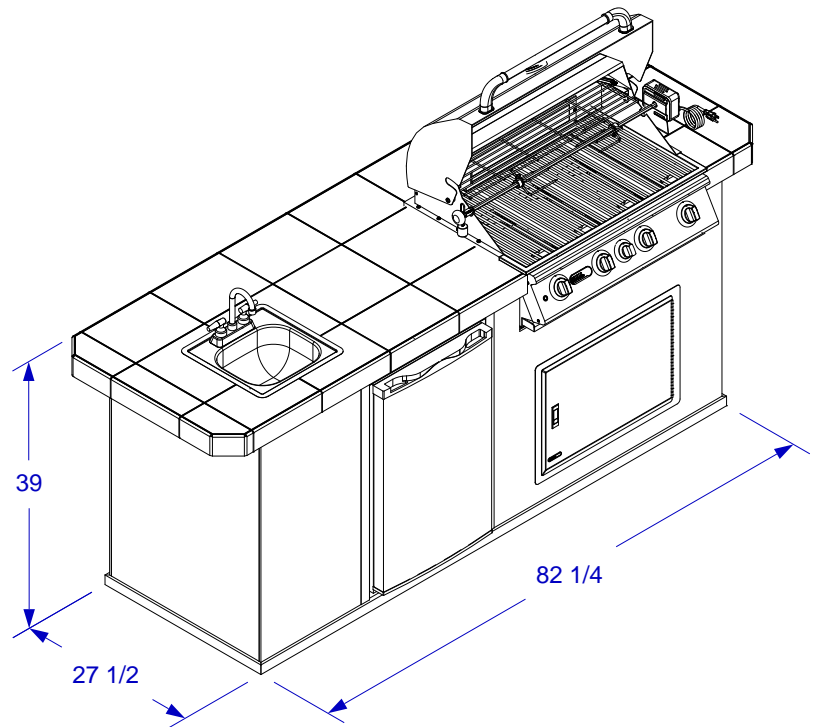
ISOMETRIC VIEW
