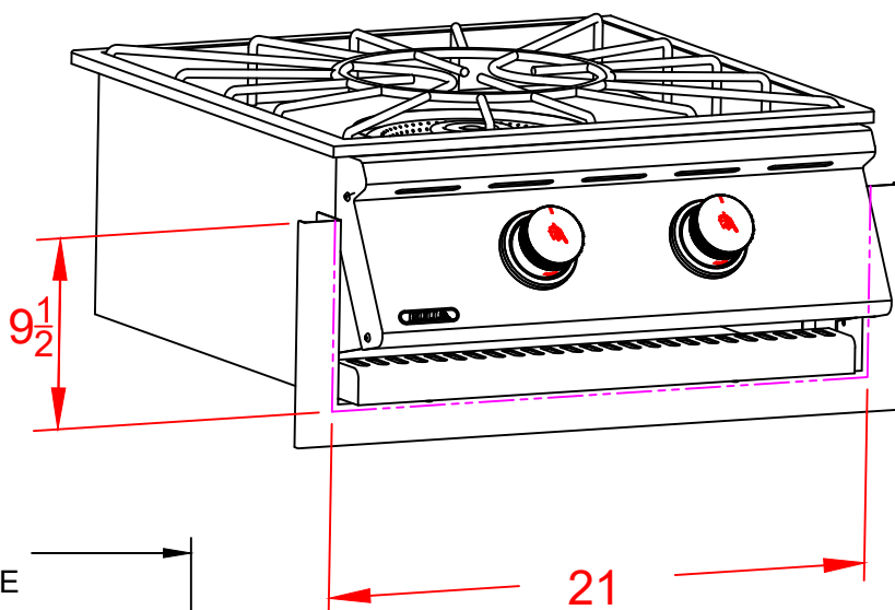
PERSPECTIVE VIEW WITH INSTALLATION CUT OUT DIMENSIONS (POWER BURNER SOLD SEPARATELY)
