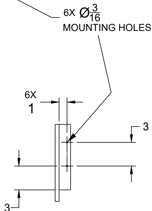
SIDE VIEW MOUNTING HOLES DIMENSIONS APPLY TO BOTH SIDES OF FRAME
