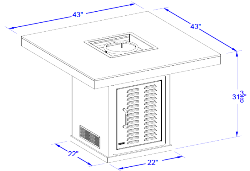
PERSPECTIVE VIEW
