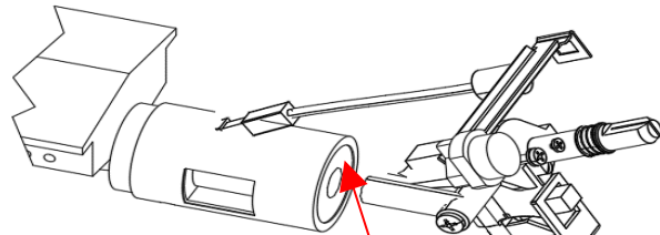
INCORRECT POSITION NOTE GAP BETWEEN BURNER TUBE AND BURNER ORIFICE
