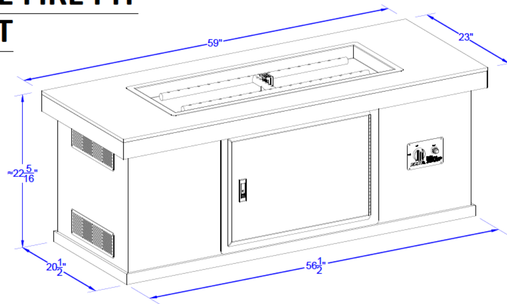
PERSPECTIVE VIEW
