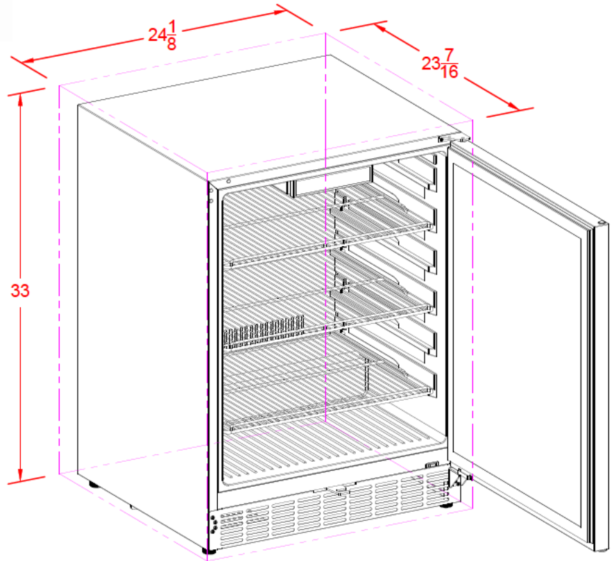
PERSPECTIVE VIEW
